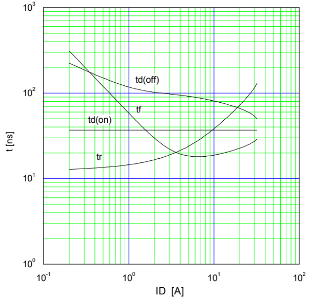
Typical Switching Characteristics vs. I D t=f(I_D):V_{cc}=300V, V_{GS}=10V, R_G=18\text{ }\Omega
