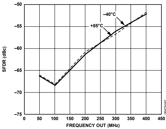
Figure 8. SFDR vs. Temperature
