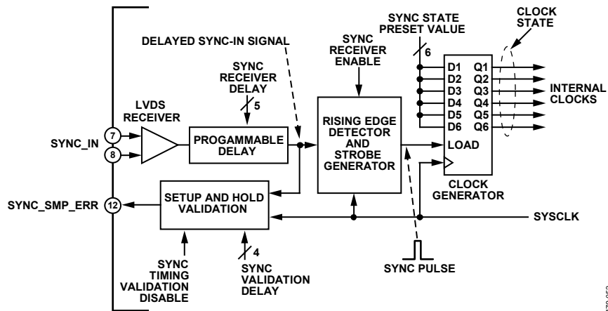
Figure 51. Sync Receiver Diagram
