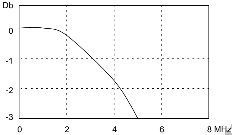
Figure-9 2X U/V filter frequency response/passband
