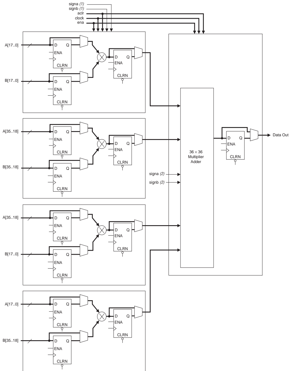
Figure 2–36. 36^\circ 36 Multiplier Mode
