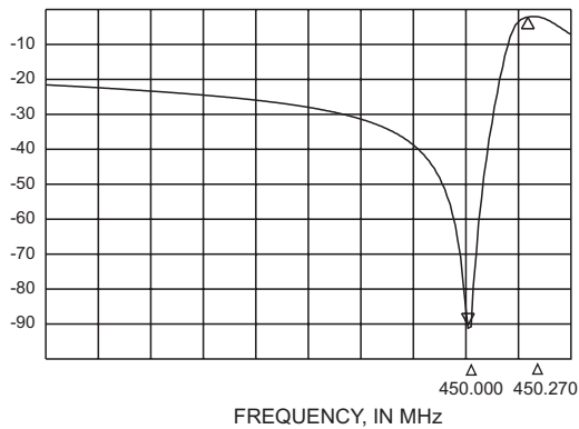
FVN15-3N • TYPICAL RESPONSE CURVES 270 KHz split
