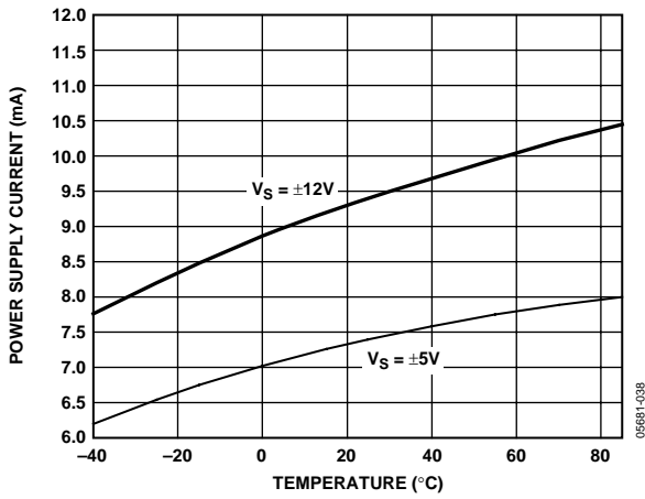
Figure 34. Power Supply Current vs. Temperature
