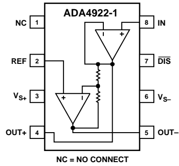
Figure 4. Pin Configuration
