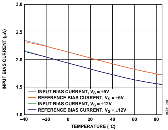
Figure 35. Input Bias Current vs. Temperature
