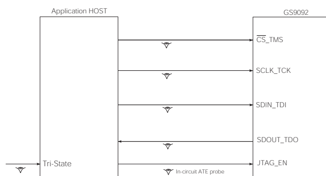
Figure 3-16: System JTAG
