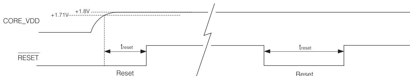
Figure 3-17: Reset pulse
