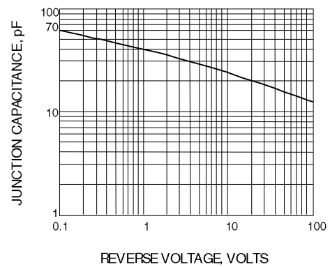
Fig. 6-TYPICAL JUNCTION CAPACITANCE
