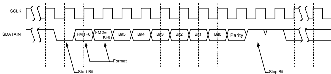
Fig. 3.2.1a: Serial interface receive timings (ASCII mode)
