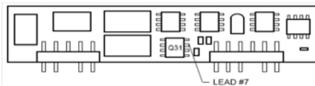
Figure 28. Temperature Measurement Location.
