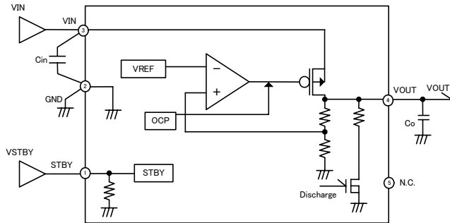
Fig.1 BLOCK DIAGRAM and APPLICATION CIRCUIT
