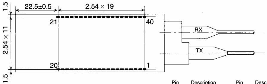
Bottom View
