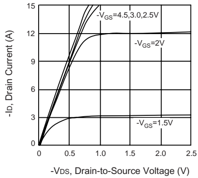
Figure 1. Output Characteristics
