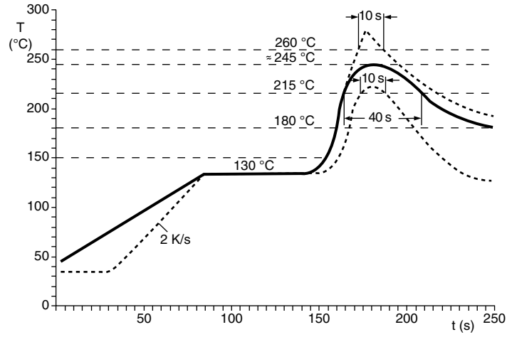
Fig. 6 - Soldering Reflow with Sn Solder
