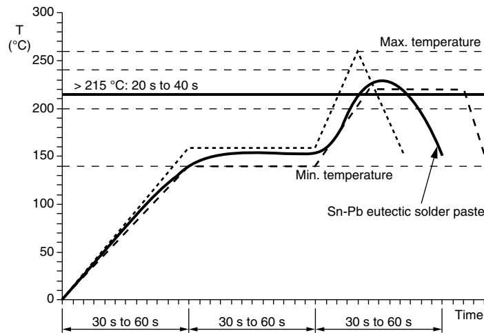
Fig. 5 - Soldering IR Reflow with SnPb Solder
