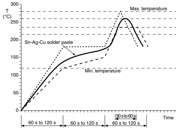
Fig. 7 - Soldering IR Reflow with SnAgCu Solder
