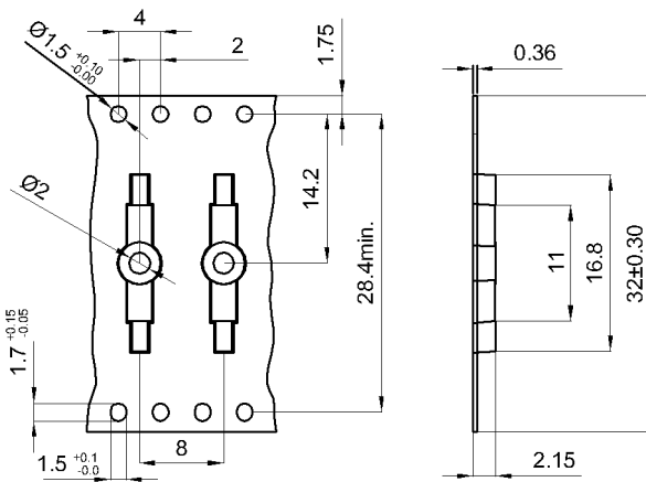
TAPE and REEL
