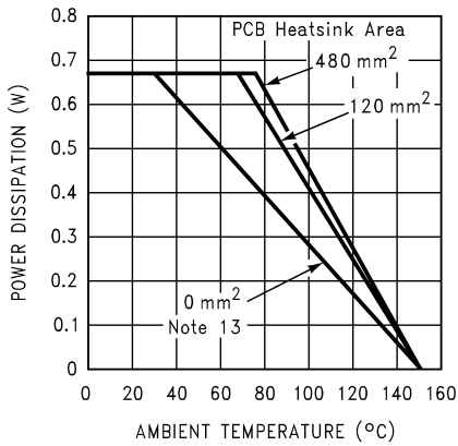
Power Derating - 9 bump μSMD ( P_{DMAX} = 670mW )
