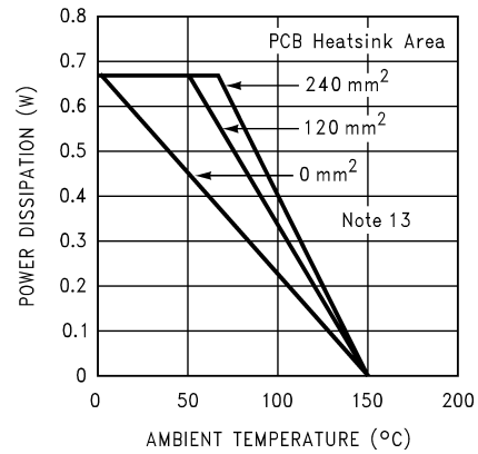
Power Derating - 8 bump μSMD ( P_{DMAX} = 670mW )
