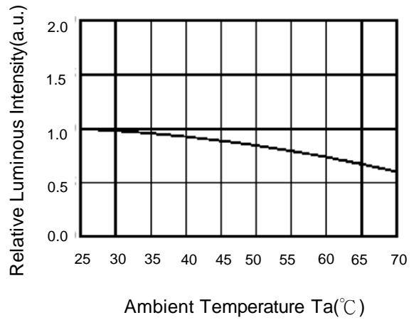
Fig.4 Relative Intensity vs. Ambient Temp
