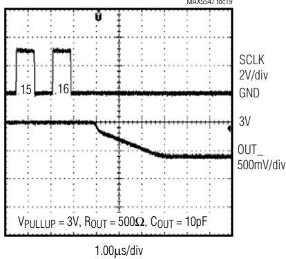
SETTLING TIME (FULL-SCALE POSITIVE STEP) ( I_{OUT} = 1.2mA )
