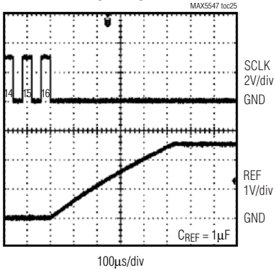
INTERNAL REFERENCE POWER-UP
