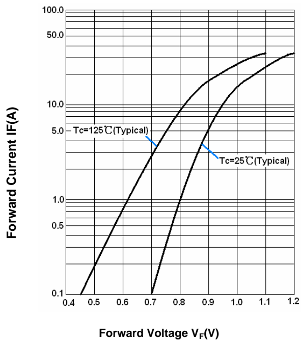
Fig.4 Forward Voltage
