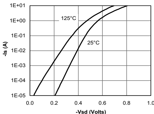
Figure 6: Body-Diode Characteristics
