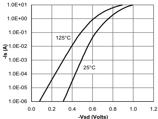
Figure 6: Body-Diode Characteristics
