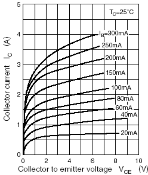
Fig.3 Static Characteristic
