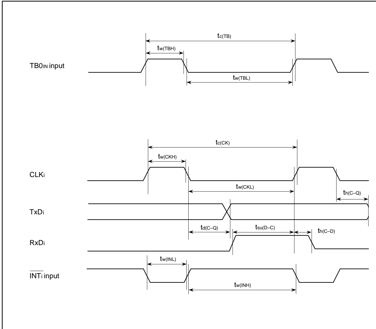
Figure 5.8.1 Timing diagram
