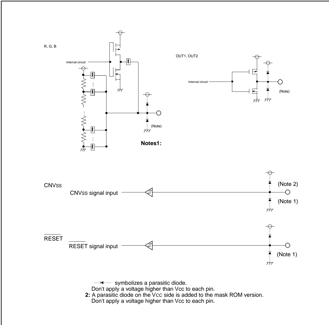
Figure 2.17.4 I/O pins
