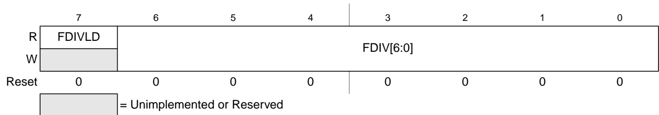
Figure 8-5. Flash Clock Divider Register (FCLKDIV)
