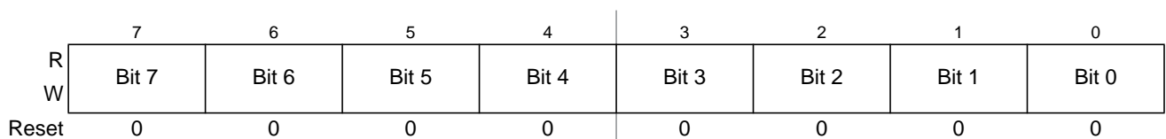
Figure 26-24. Timer Input Capture/Output Compare Register 2 Low (TC2)
