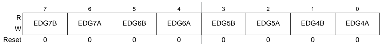
Figure 26-13. Timer Control Register 3 (TCTL3)
