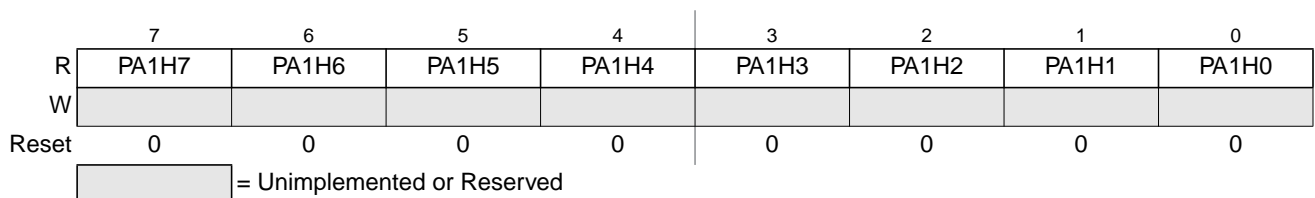
Figure 26-54. 8-Bit Pulse Accumulators Holding Register 1 (PA1H)
