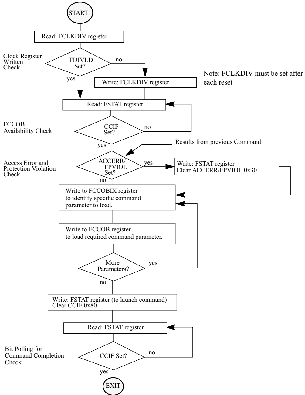
Figure 7-26. Generic Flash Command Write Sequence Flowchart
