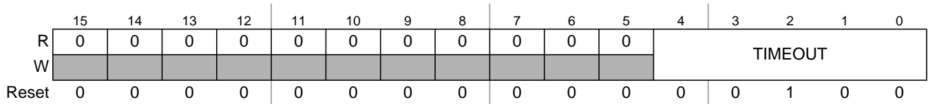
Figure 13-31. System Memory Access Time-Out Register (SYMATOR)
