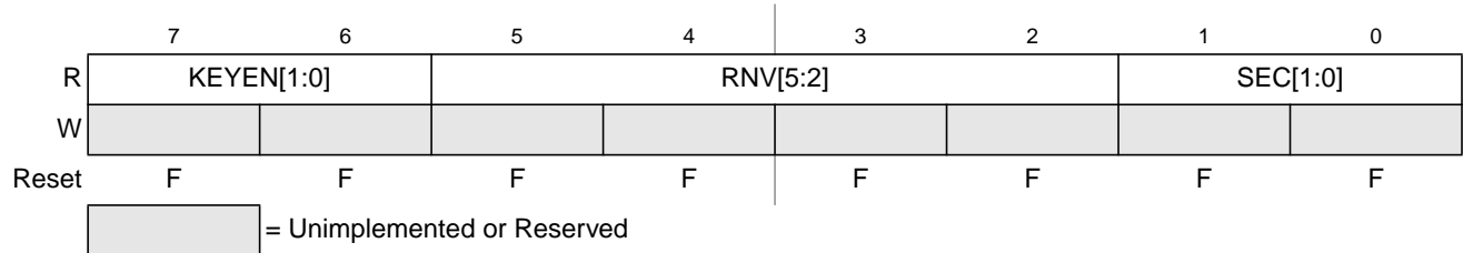
Figure 7-6. Flash Security Register (FSEC)
