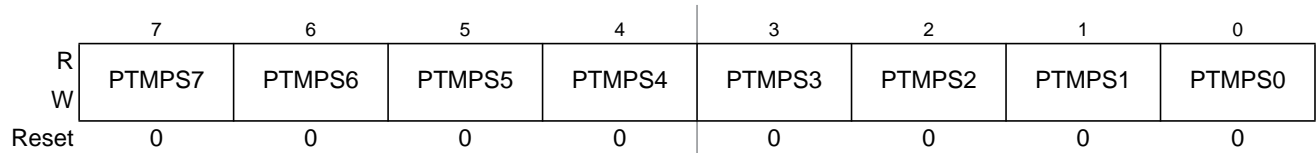
Figure 26-49. Precision Timer Modulus Counter Prescaler Select Register (PTMCPSR)
