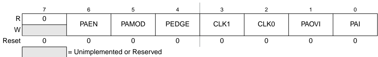
Figure 26-35. 16-Bit Pulse Accumulator Control Register (PACTL)
