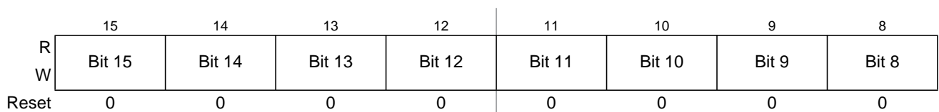
Figure 26-25. Timer Input Capture/Output Compare Register 3 High (TC3)
