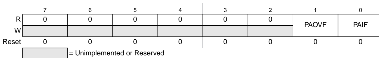
Figure 26-36. Pulse Accumulator A Flag Register (PAFLG)
