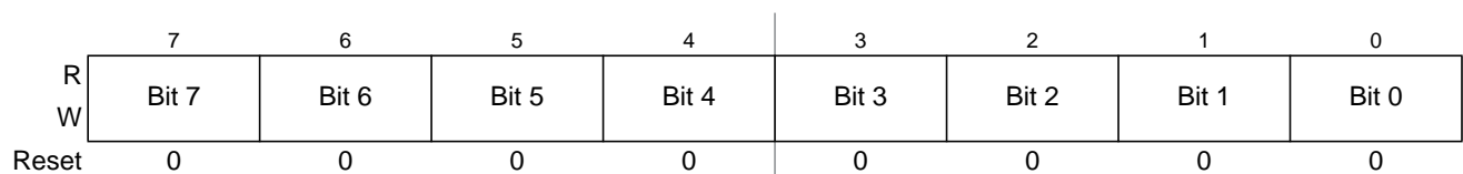
Figure 26-30. Timer Input Capture/Output Compare Register 5 Low (TC5)
