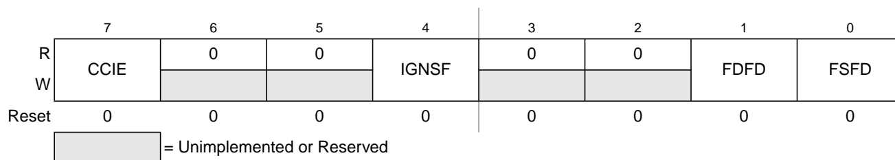
Figure 7-9. Flash Configuration Register (FCNFG)
