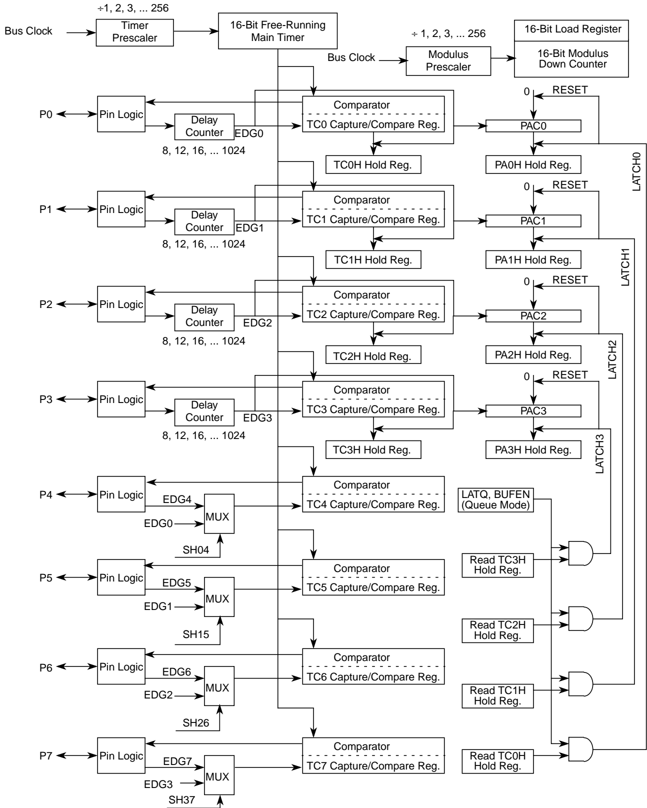
Figure 26-69. Detailed Timer Block Diagram in Queue Mode when PRNT = 1
