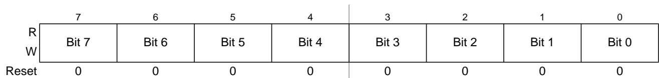
Figure 26-28. Timer Input Capture/Output Compare Register 4 Low (TC4)
