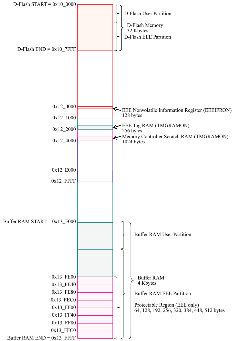
Figure 8-3. EEE Resource Memory Map
