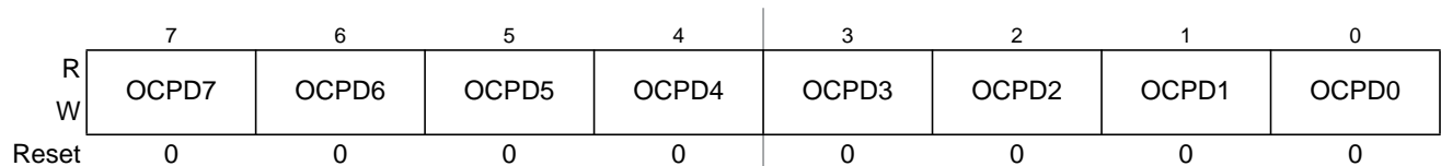
Figure 26-47. Output Compare Pin Disconnect Register (OCPD)
