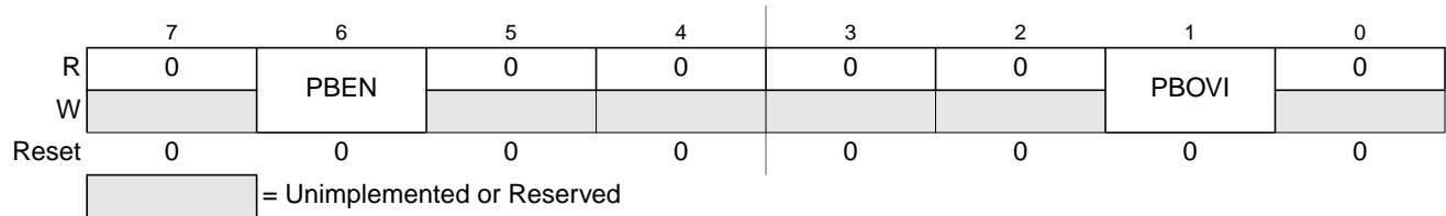
Figure 26-50. 16-Bit Pulse Accumulator B Control Register (PBCTL)
