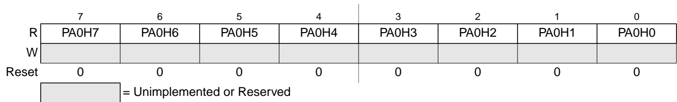
Figure 26-55. 8-Bit Pulse Accumulators Holding Register 0 (PA0H)
