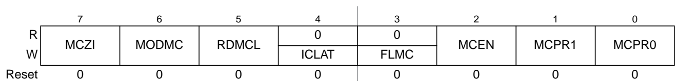
Figure 26-41. 16-Bit Modulus Down-Counter Control Register (MCCTL)
