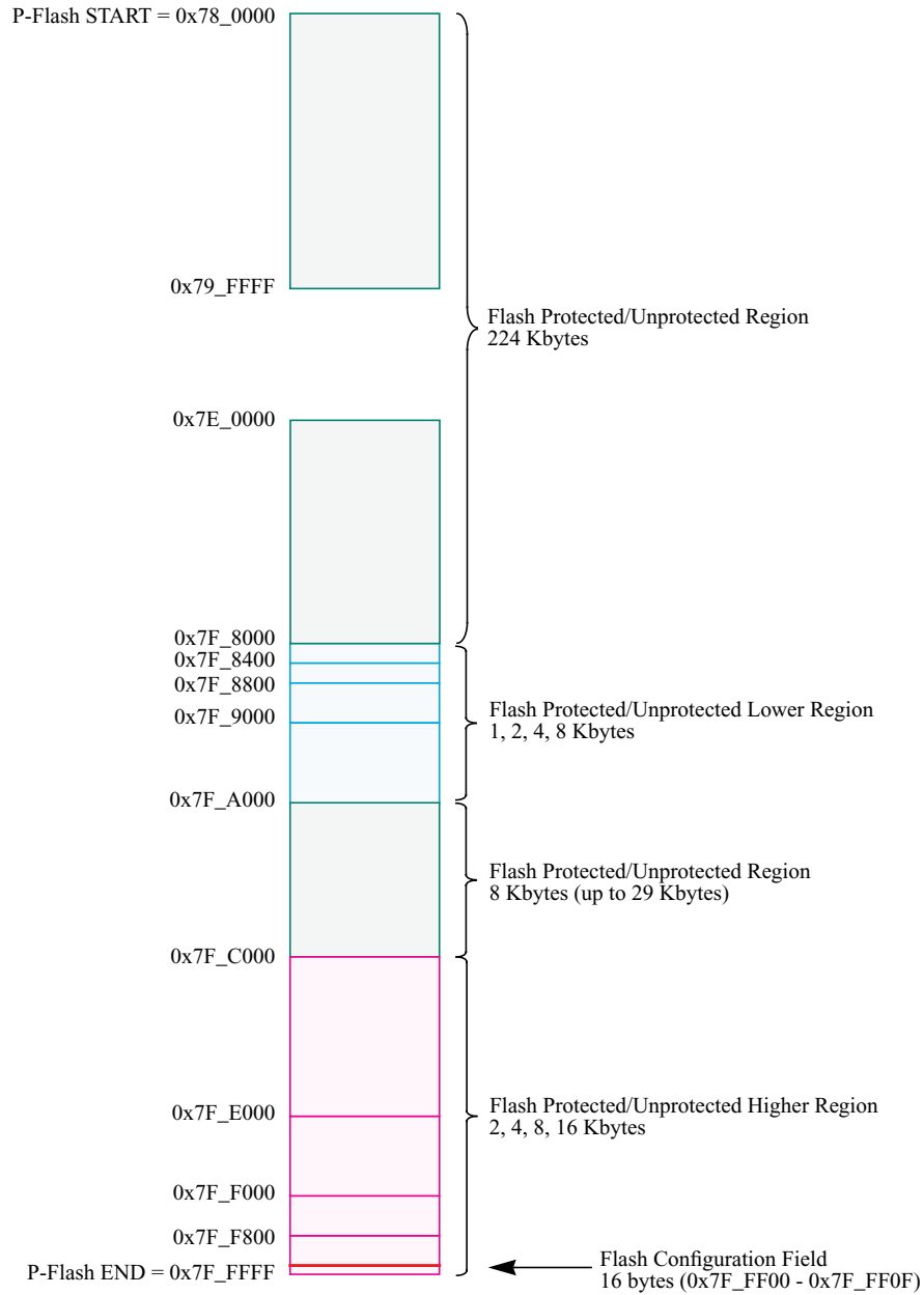
Figure 7-2. P-Flash Memory Map
