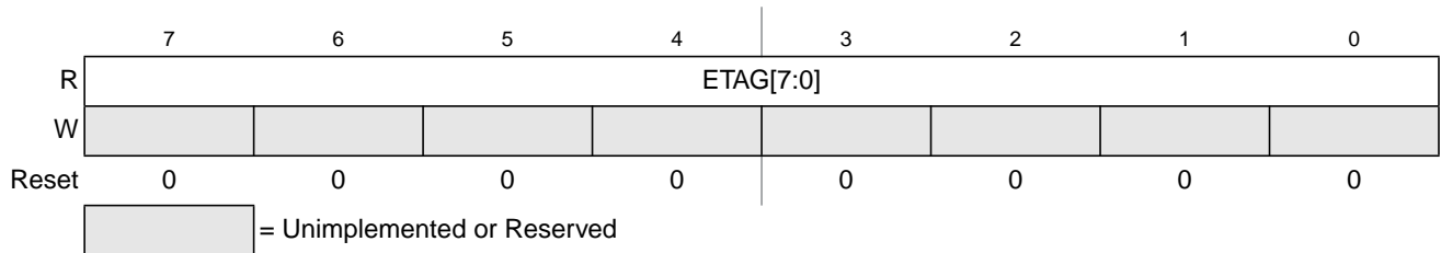
Figure 7-19. EEE Tag Counter Low Register (ETAGLO)
