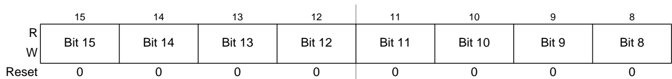
Figure 26-29. Timer Input Capture/Output Compare Register 5 High (TC5)
