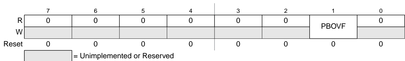
Figure 26-51. Pulse Accumulator B Flag Register (PBFLG)
