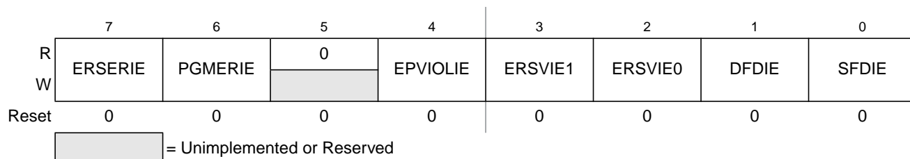
Figure 7-10. Flash Error Configuration Register (FERCNFG)
