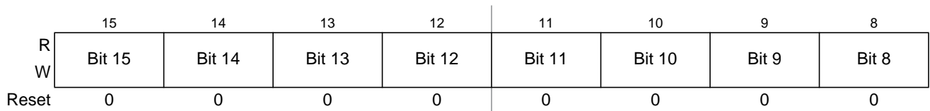
Figure 26-21. Timer Input Capture/Output Compare Register 1 High (TC1)
