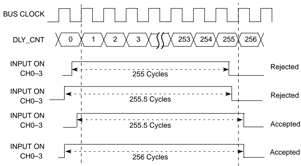
Figure 26-73. Channel Input Validity with Delay Counter Feature
