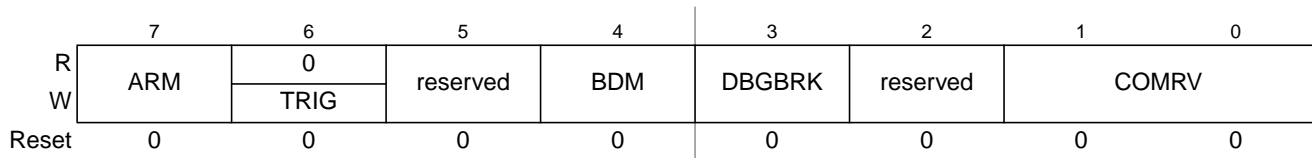
Figure 16-3. Debug Control Register (DBGCR1)
