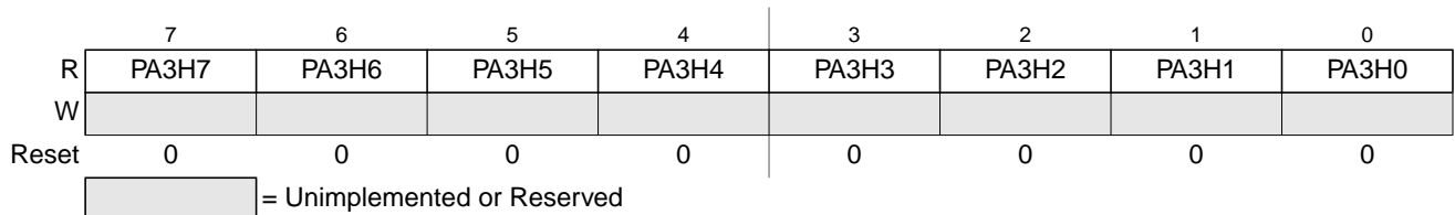
Figure 26-52. 8-Bit Pulse Accumulators Holding Register 3 (PA3H)
