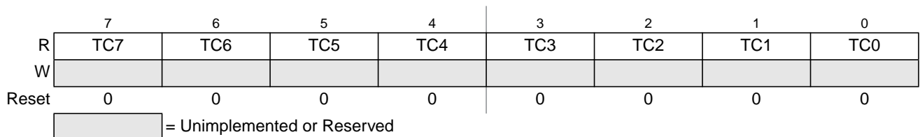
Figure 26-59. Timer Input Capture Holding Register 0 Low (TC0L)
