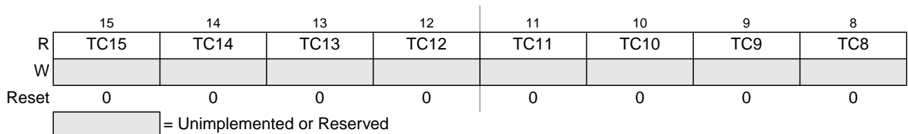
Figure 26-58. Timer Input Capture Holding Register 0 High (TC0H)
