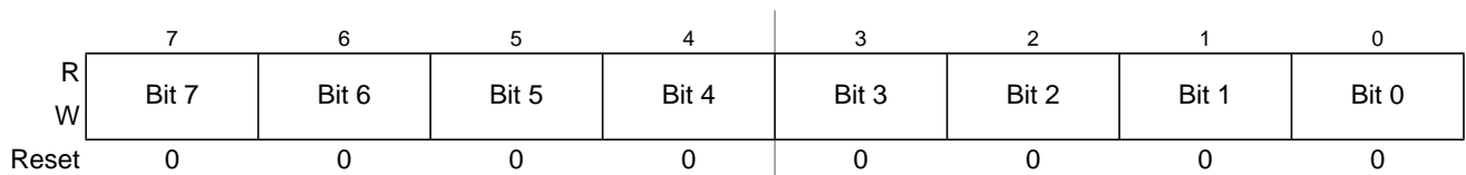
Figure 26-22. Timer Input Capture/Output Compare Register 1 Low (TC1)
