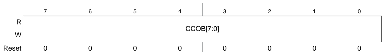
Figure 7-17. Flash Common Command Object Low Register (FCCOBLO)
