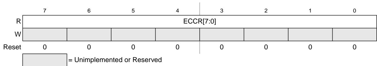
Figure 7-21. Flash ECC Error Results Low Register (FECCRLO)
