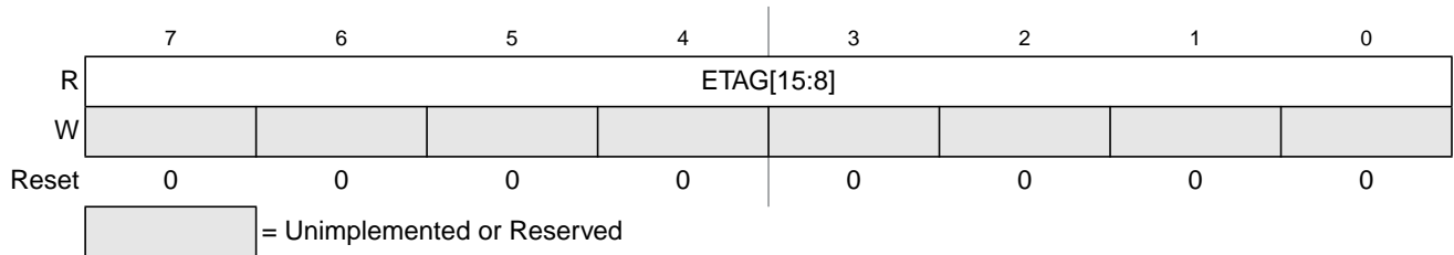
Figure 7-18. EEE Tag Counter High Register (ETAGHI)
