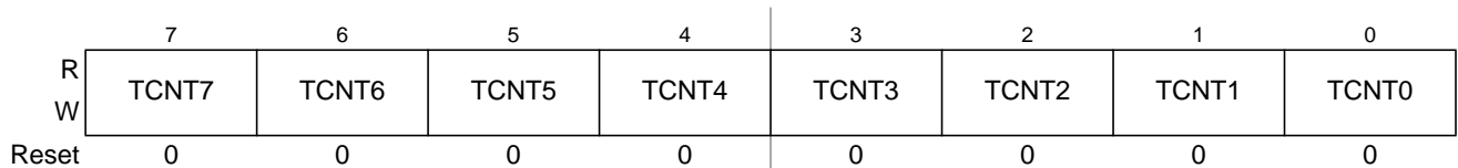
Figure 26-8. Timer Count Register Low (TCNT)
