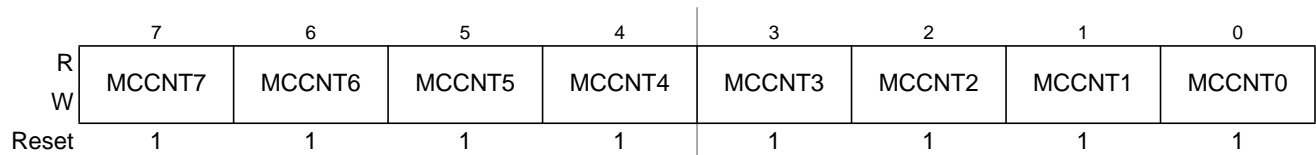
Figure 26-57. Modulus Down-Counter Count Register Low (MCCNT)
