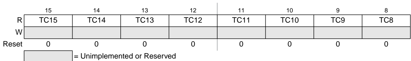
Figure 26-60. Timer Input Capture Holding Register 1 High (TC1H)
