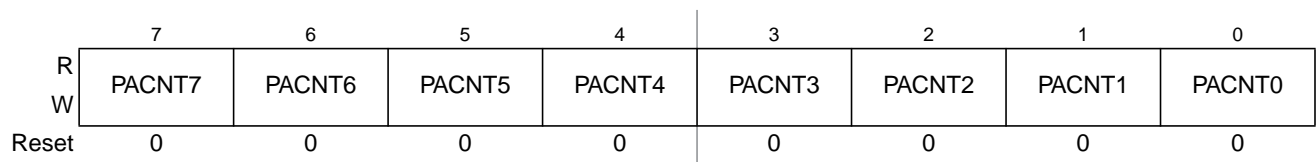
Figure 26-40. Pulse Accumulators Count Register 0 (PACN0)
