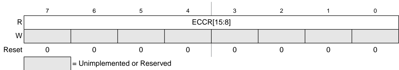
Figure 7-20. Flash ECC Error Results High Register (FECCRHI)
