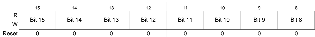
Figure 26-19. Timer Input Capture/Output Compare Register 0 High (TC0)
