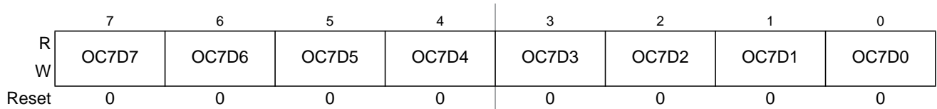
Figure 26-6. Output Compare 7 Data Register (OC7D)
