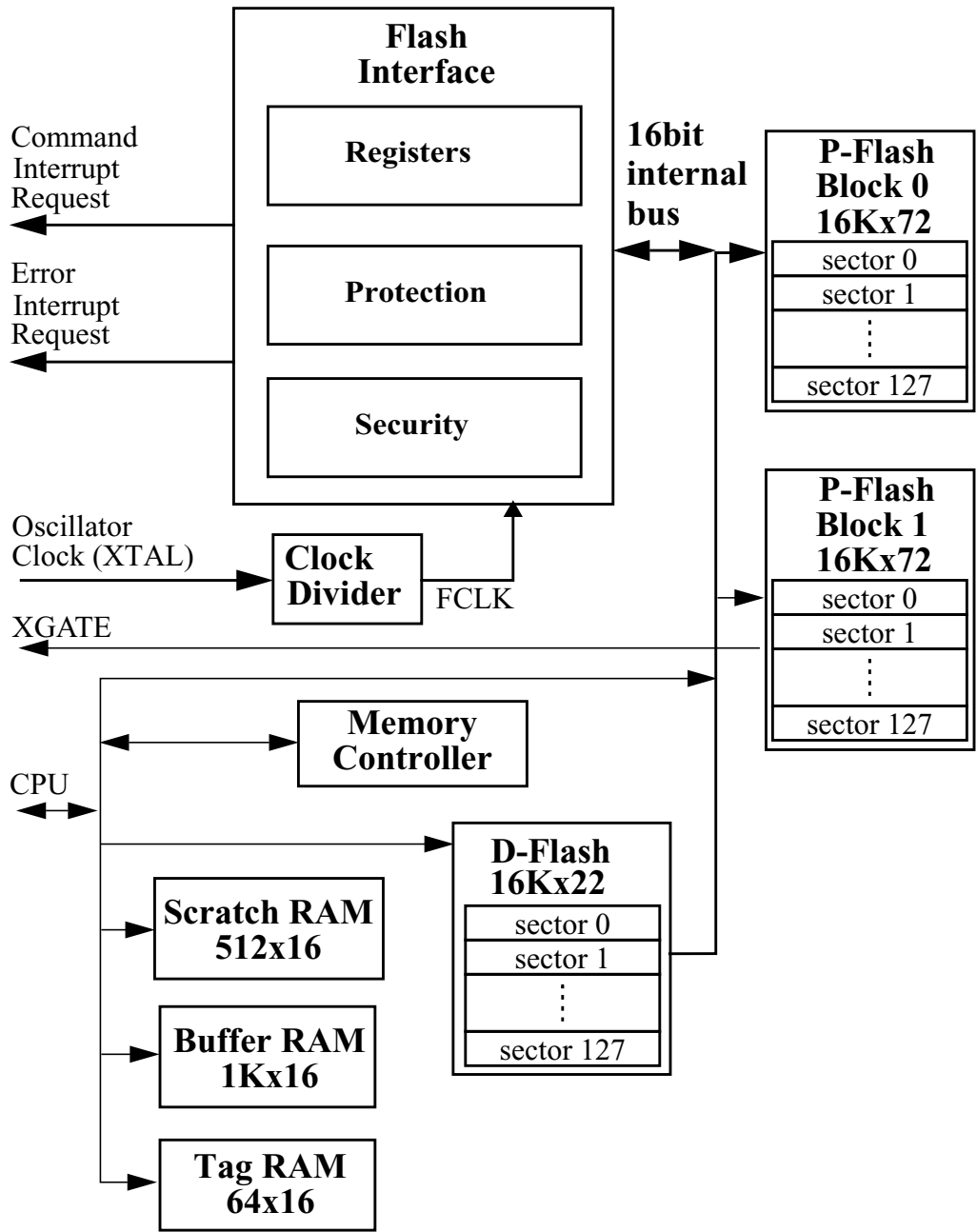
Figure 7-1. FTM256K2 Block Diagram
