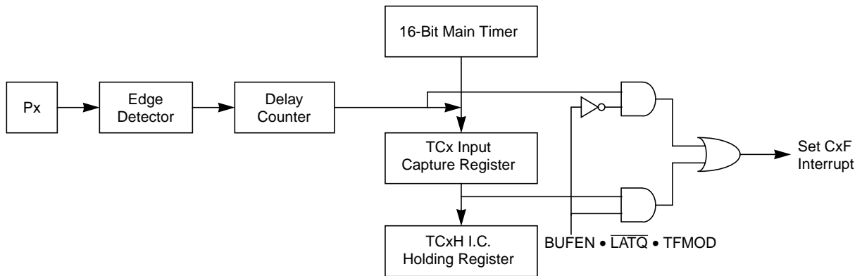
Figure 26-72. Block Diagram for Port 7 with Output Compare/Pulse Accumulator A
