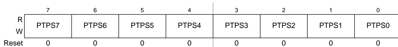
Figure 26-48. Precision Timer Prescaler Select Register (PTPSR)
