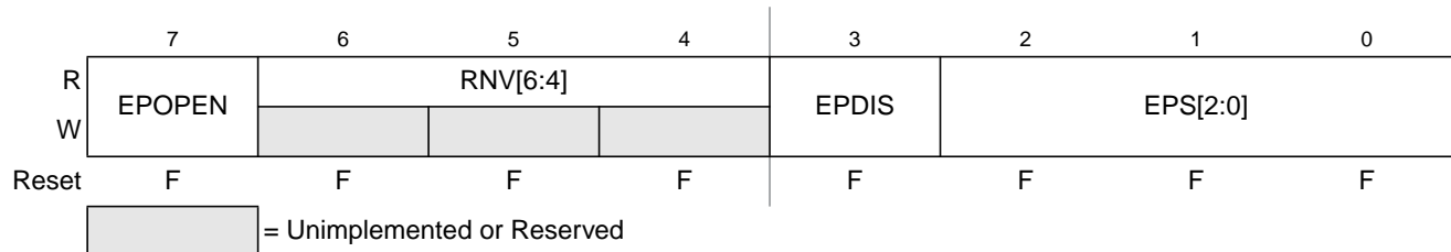
Figure 7-15. EEE Protection Register (EPROT)
