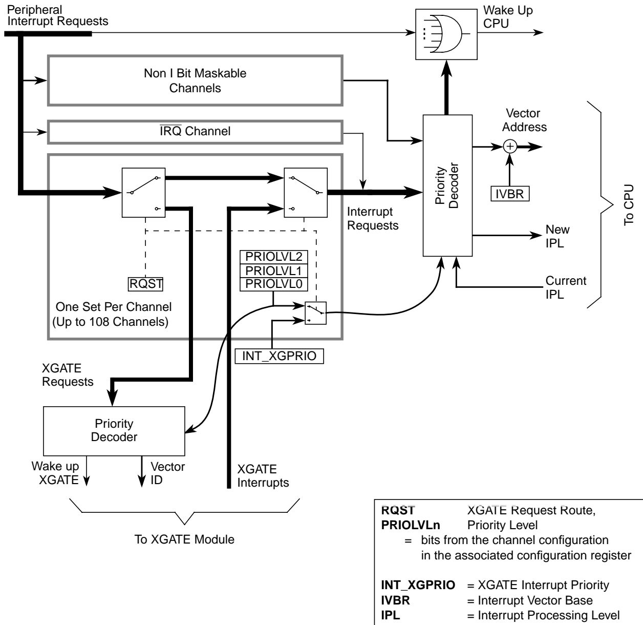
Figure 6-1. INT Block Diagram
