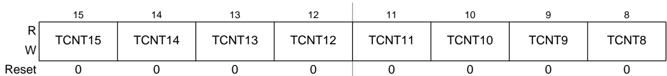
Figure 26-7. Timer Count Register High (TCNT)
