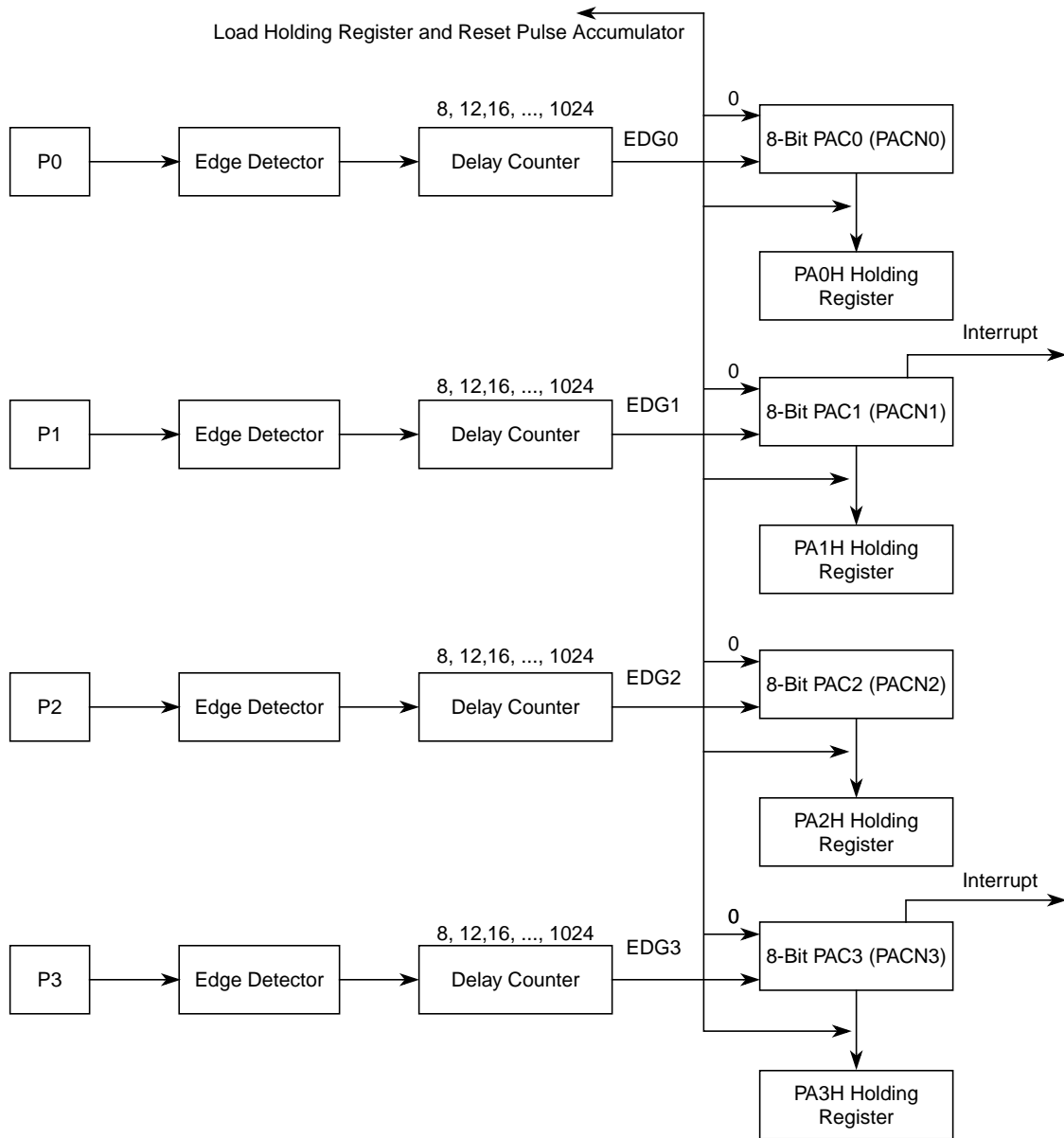
Figure 26-70. 8-Bit Pulse Accumulators Block Diagram
