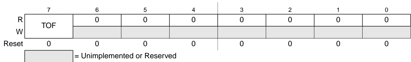
Figure 26-18. Main Timer Interrupt Flag 2 (TFLG2)
