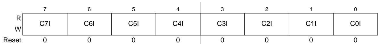
Figure 26-15. Timer Interrupt Enable Register (TIE)
