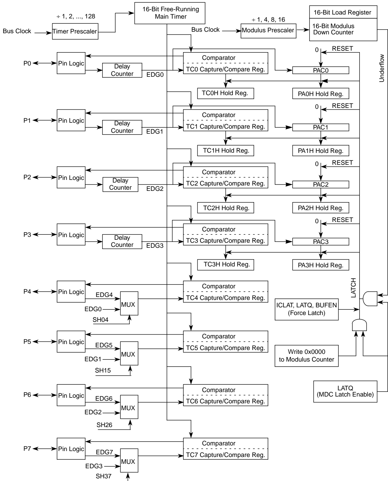
Figure 26-66. Detailed Timer Block Diagram in Latch Mode when PRNT = 0
