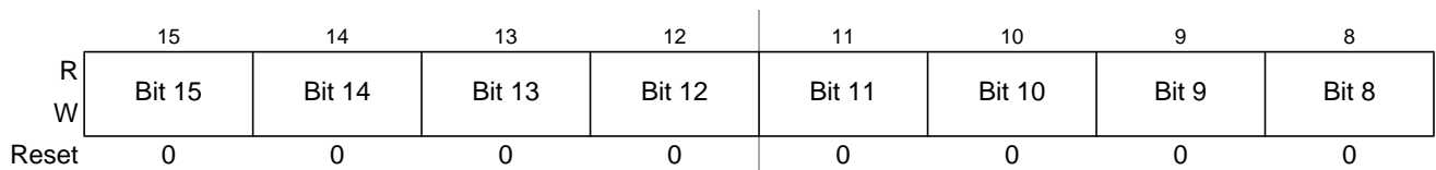
Figure 26-23. Timer Input Capture/Output Compare Register 2 High (TC2)
