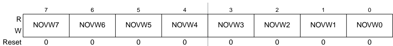
Figure 26-45. Input Control Overwrite Register (ICOVW)
