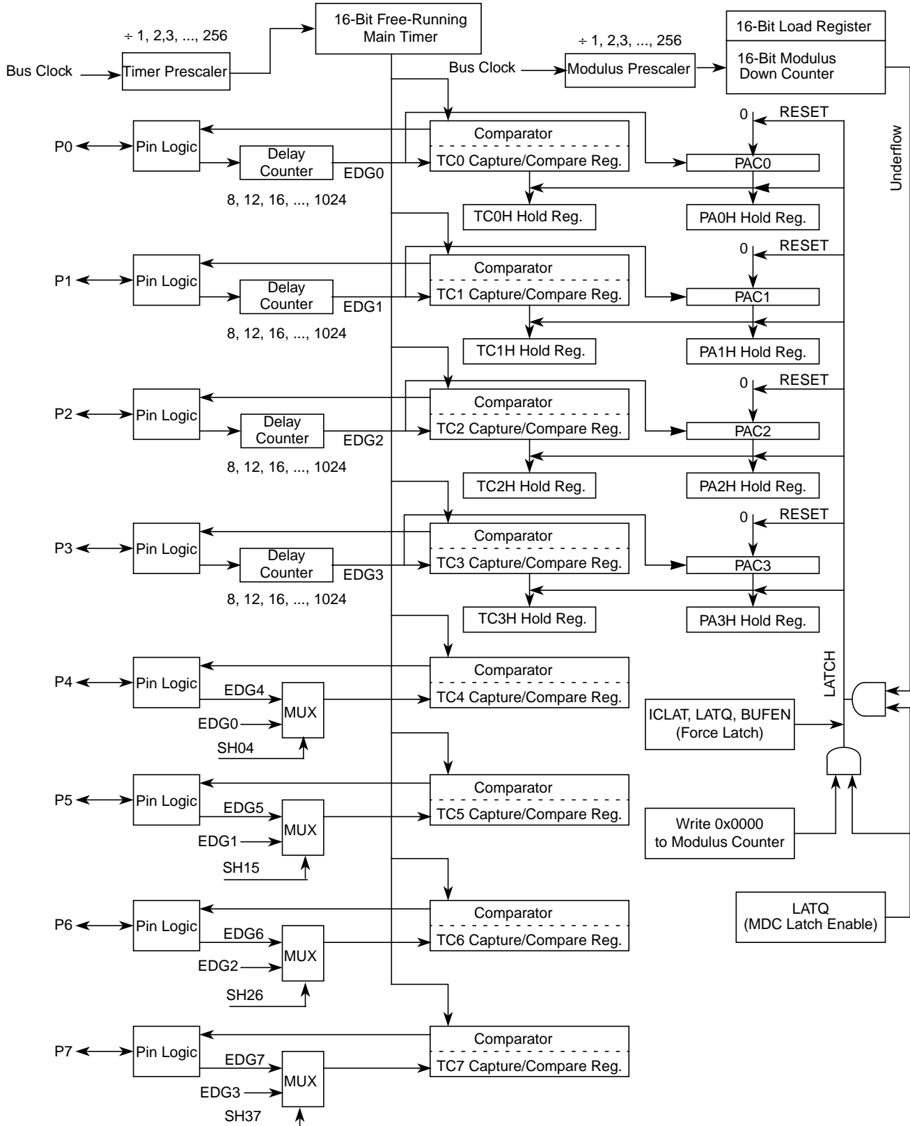
Figure 26-67. Detailed Timer Block Diagram in Latch Mode when PRNT = 1
