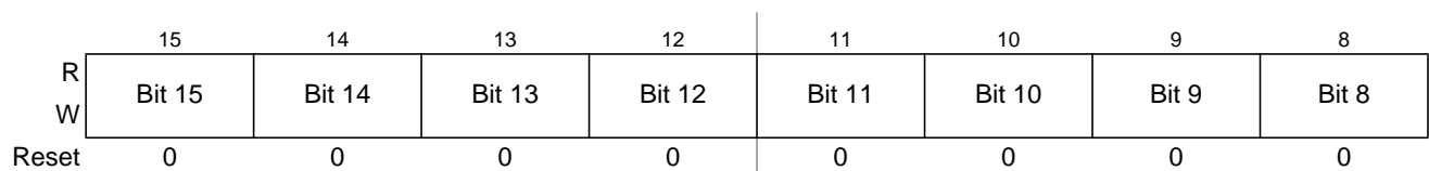
Figure 26-31. Timer Input Capture/Output Compare Register 6 High (TC6)
