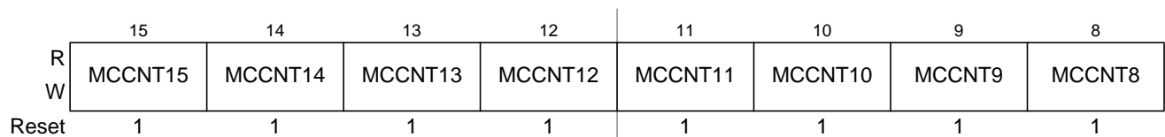
Figure 26-56. Modulus Down-Counter Count Register High (MCCNT)
