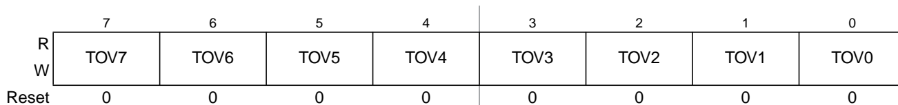
Figure 26-10. Timer Toggle On Overflow Register 1 (TTOV)
