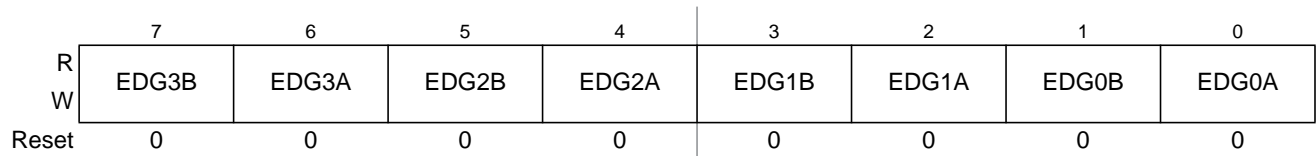
Figure 26-14. Timer Control Register 4 (TCTL4)
