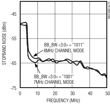
STOPBAND NOISE vs. FREQUENCY
