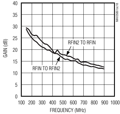
RF PORT-TO-PORT ISOLATION
