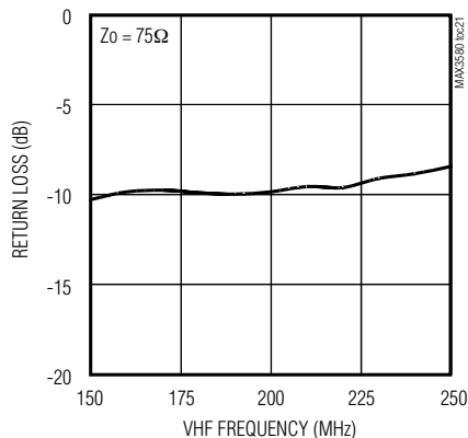
RF INPUT RETURN LOSS vs. VHF FREQUENCY
