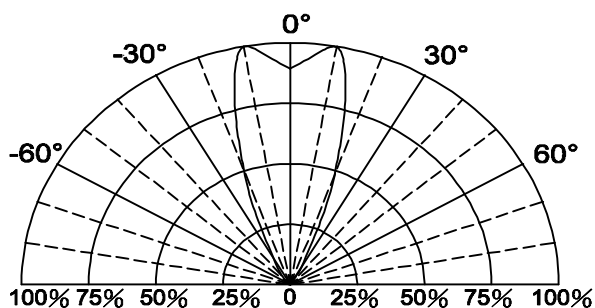
Fig.5 Directivity Radiation
