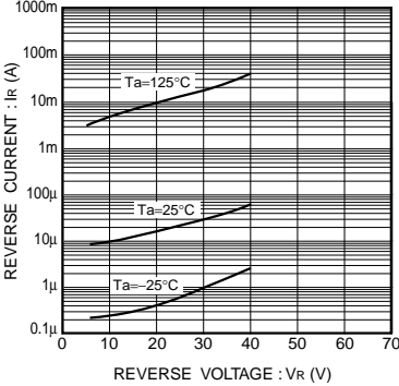
Fig.09 Reverse characteristics
