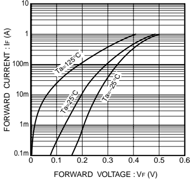
Fig.8 Forward characteristics
