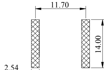
( PCB Pattern )
