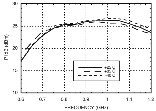
Input P1dB vs. Temperature
