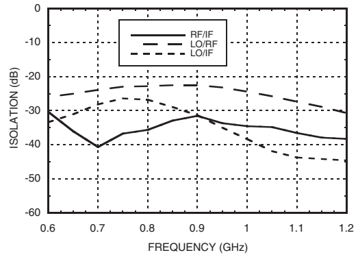
Isolation
