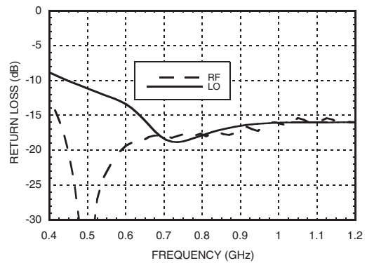
Return Loss
