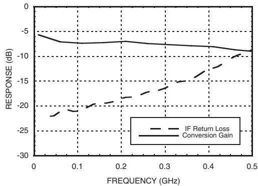
IF Bandwidth (LO = 0.8 GHz)
