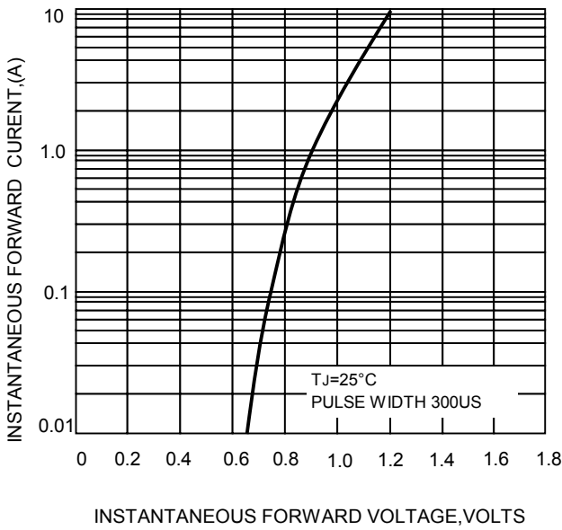
FIG.3-TYPICAL FORWARD CHARACTERISTICS
