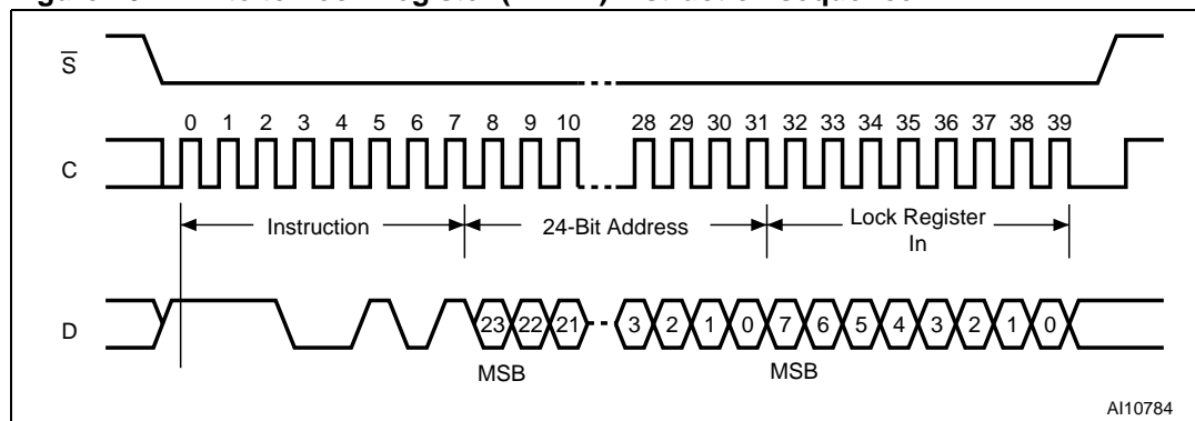
Figure 16. Write to Lock Register (WRLR) instruction sequence
