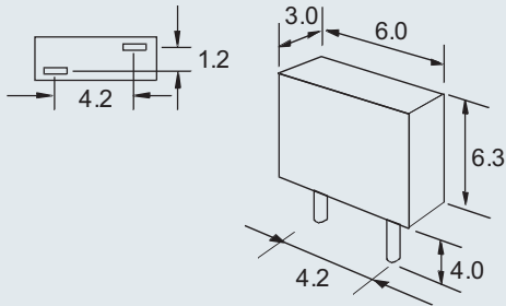
Outline and Dimensions
