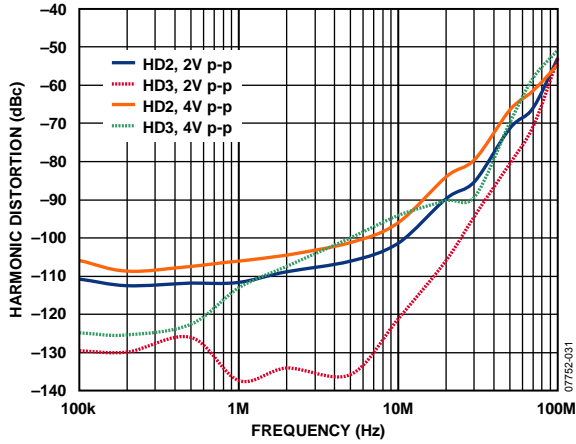
Figure 31. Harmonic Distortion vs. Frequency at Various V_{OUT,dm}
