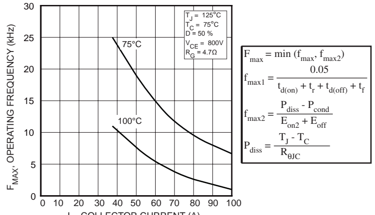
Figure 20, Operating Frequency vs Collector Current
