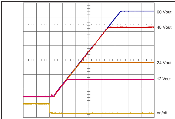
Figure 7: Turn-on transient at 36 V input; full load (20 ms/div). Ch 1: ON/OFF input (5 V/div) Ch 2-4: Vout (10 V/div)
