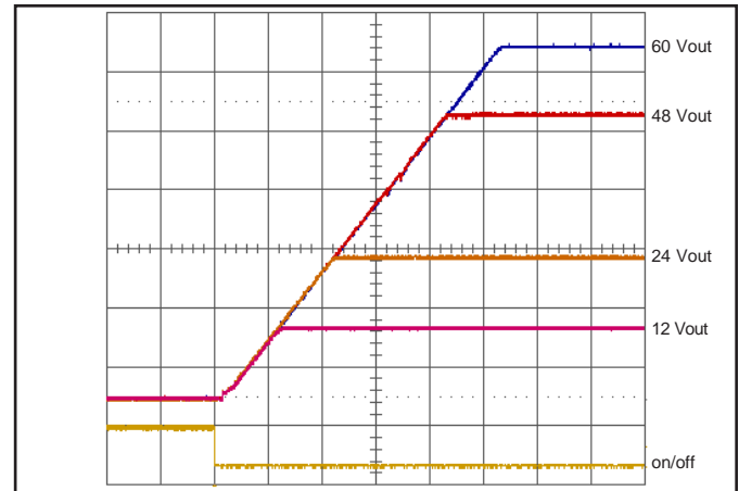
Figure 8: Turn-on transient at 36 V input; zero load (20 ms/div). Ch 1: ON/OFF input (5 V/div) Ch 2-4: Vout (10 V/div)
