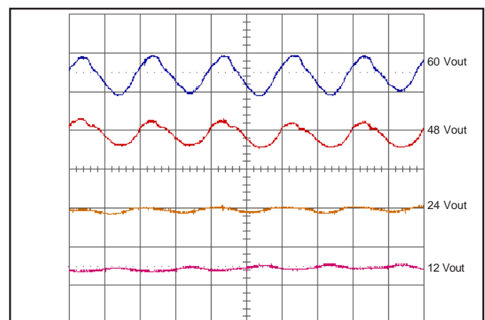
Figure 6: Output Voltage Ripple at 36 V input and rated load current (50 mV/div). Load capacitance: 100 µF electrolytic cap., Bandwidth: 20 MHz. See Figure 4.
