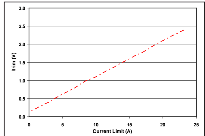
Figure 10: Current limit vs. Itrim pin voltage at 24 V input and 13.8 V output. Load capacitance: 100 \mu F electrolytic cap. C option only.
