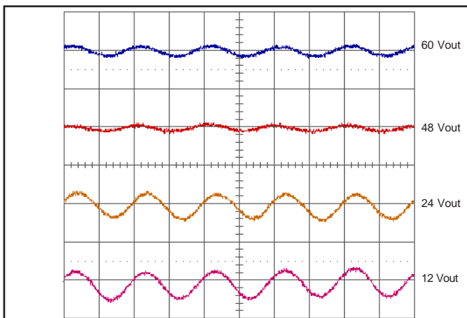
Figure 5: Input Terminal Ripple Current at 36 V input and rated load current (500 mA/div). Load capacitance: 100 µF electrolytic cap. Bandwidth: 20 MHz. See Figure 4.
