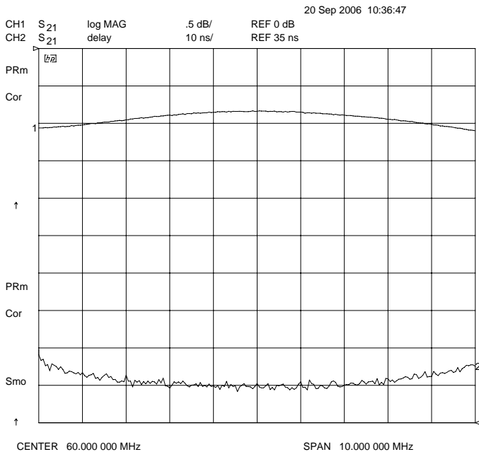
Passband Amplitude & Group Delay (0.5 dB/div and 10 nsec/div)
