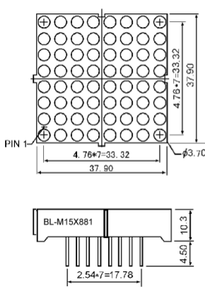
BL-M15X881 Series
