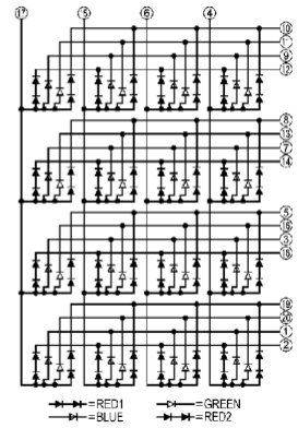
BL-M15F881
