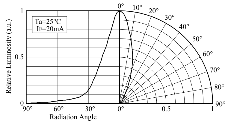
■ Directivity (NSPG310A)
