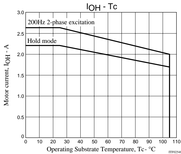
Derating curve of motor current, I_{OH} , vs. STK672-630A-E Operating substrate temperature, T_c
