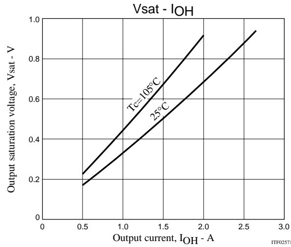
STK672-630A-E Output saturation voltage, V_{sat} - Output current, I_{OH}
