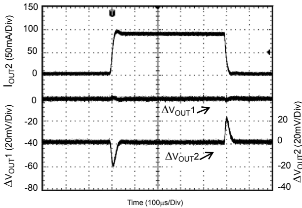
Figure 38. Cross Talk 1
