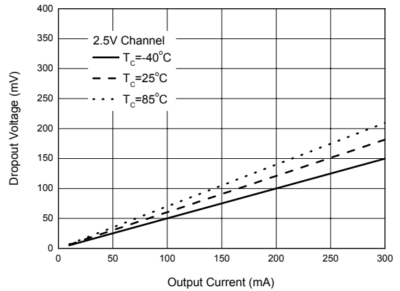
Figure 23. Dropout Voltage vs. Output Current
