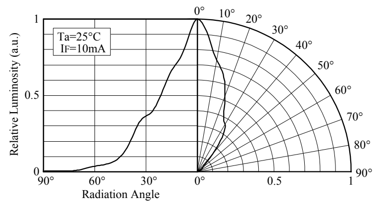
■ Directivity (NSPE520S)
