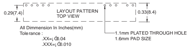
Figure 8. Recommended VPOL16A-12W-SIP Footprint
