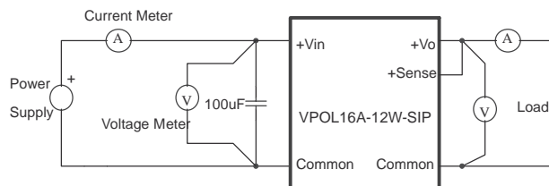
Figure 13. VPOL16A-12W-SIP Series Test Setup
