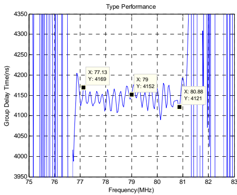
Group Delay Variation(f0±1.88MHz)
