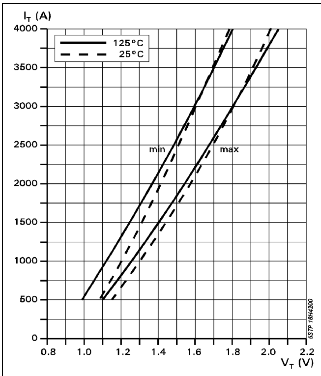
Fig. 2 On-state characteristics.
