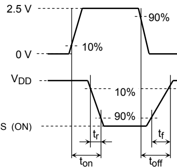
(c) V_{OUT}
