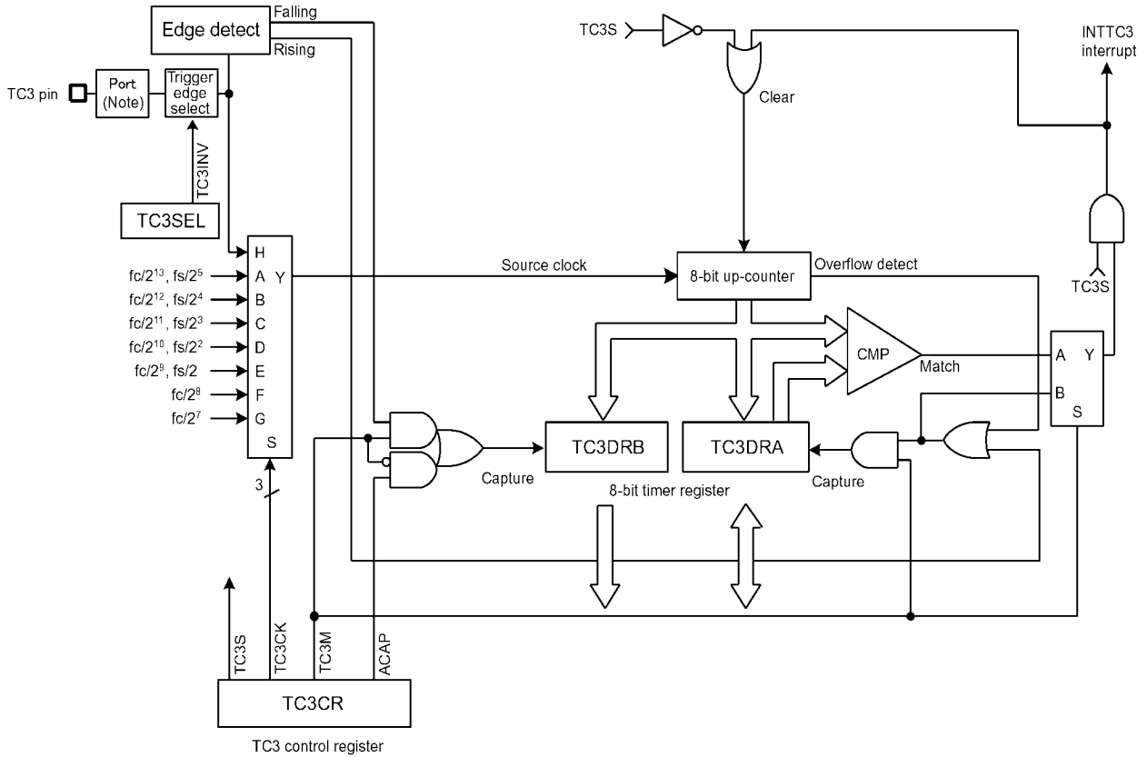
Figure 10-1 TimerCounter 3 (TC3)
