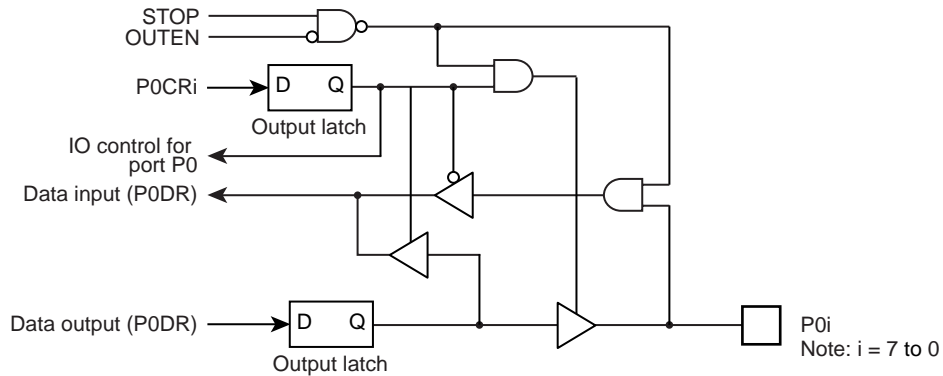
Figure 5-2 Port P0
