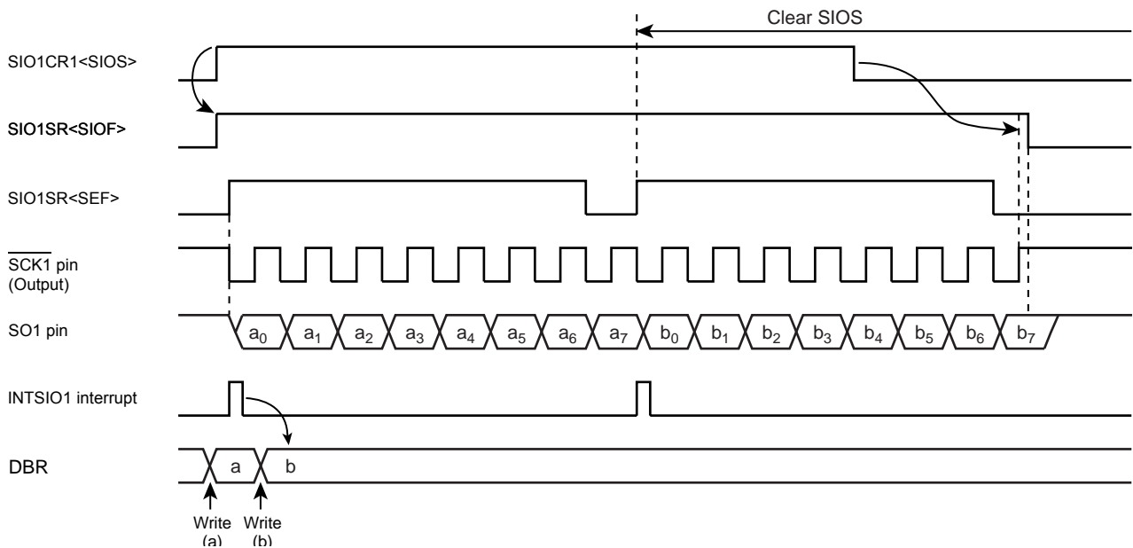
Figure 15-7 Transfer Mode (Example: 8bit, 1word transfer, Internal clock)
