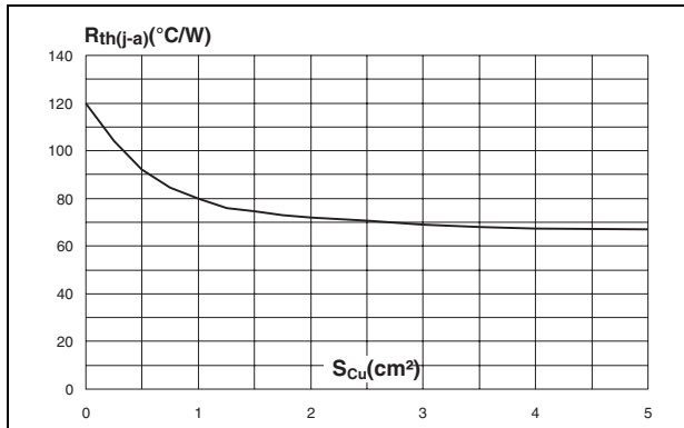
Figure 13. Thermal resistance junction to ambient versus copper surface under each lead - Epoxy printed circuit board FR4, \epsilon_{Cu} = 35 \mu m (SMA)
