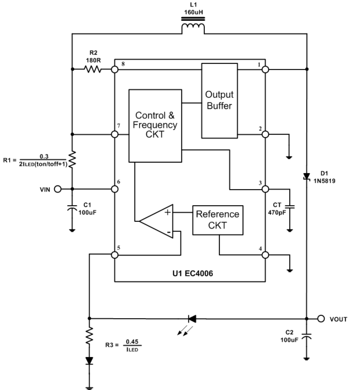
Figure 9. Step-Up type
