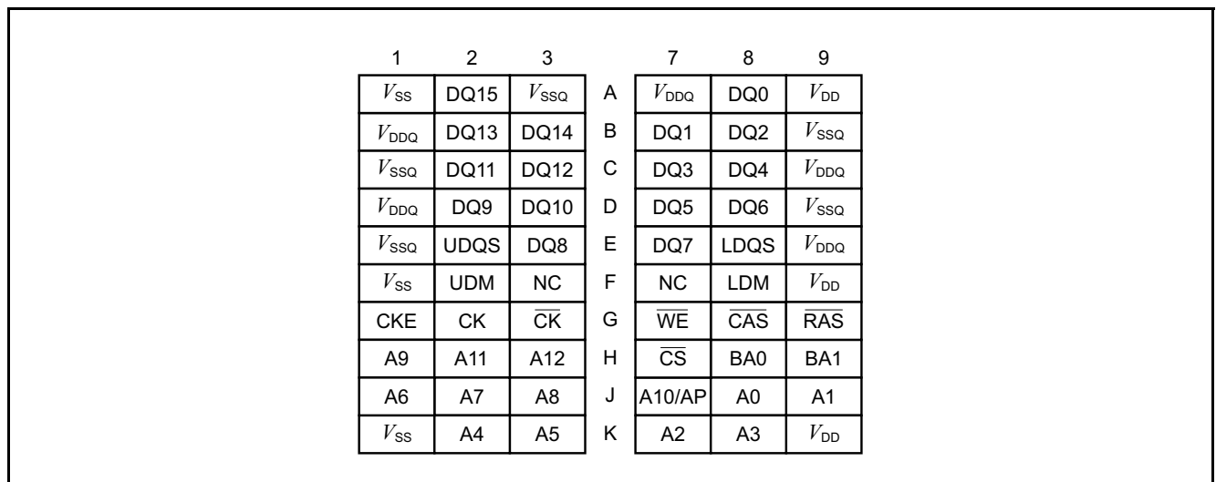
Figure 1 Standard Ballout 512-Mbit DDR Mobile-RAM (Top View)
